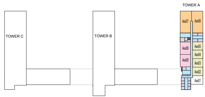
LEVEL 12,24,36,48
