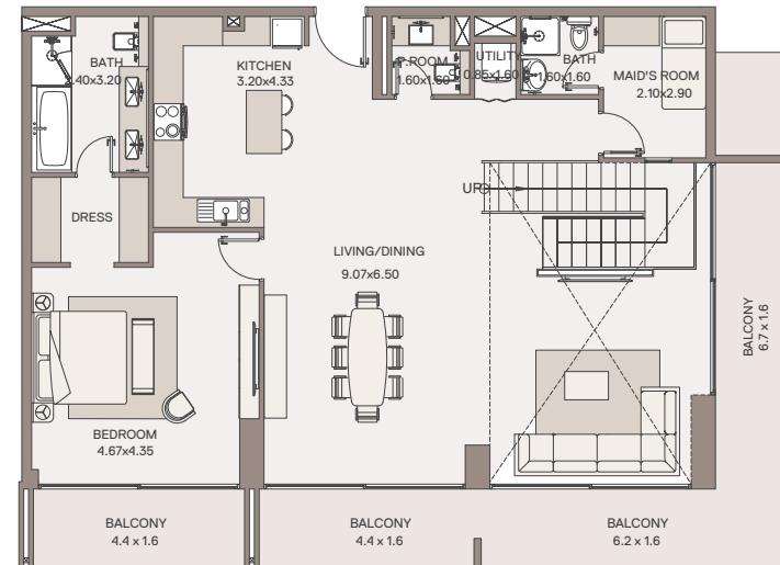
9 th floor
